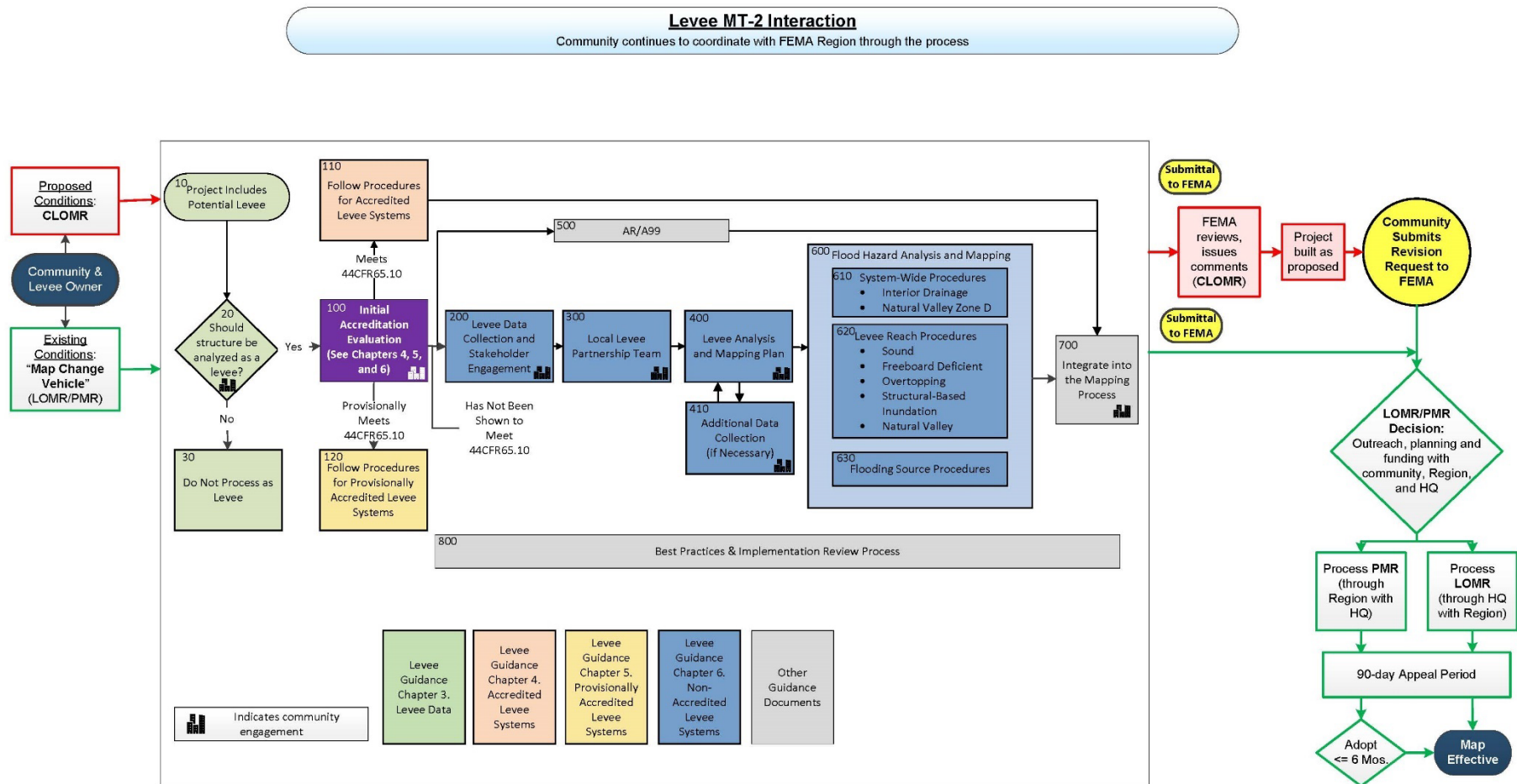
Figure 5. Levee Analysis and Mapping Procedures Workflow
