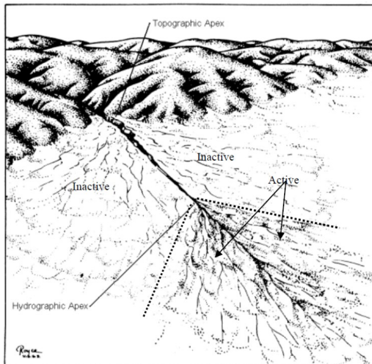
Figure 4. Active and Inactive Alluvial Fan Flow Paths
